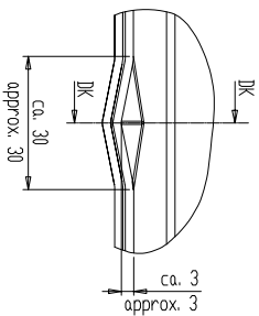
Detail Kerbe Detail notch
