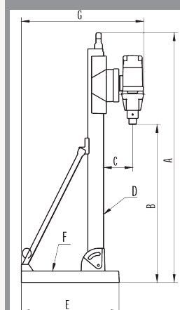
Dimensions (mm)
